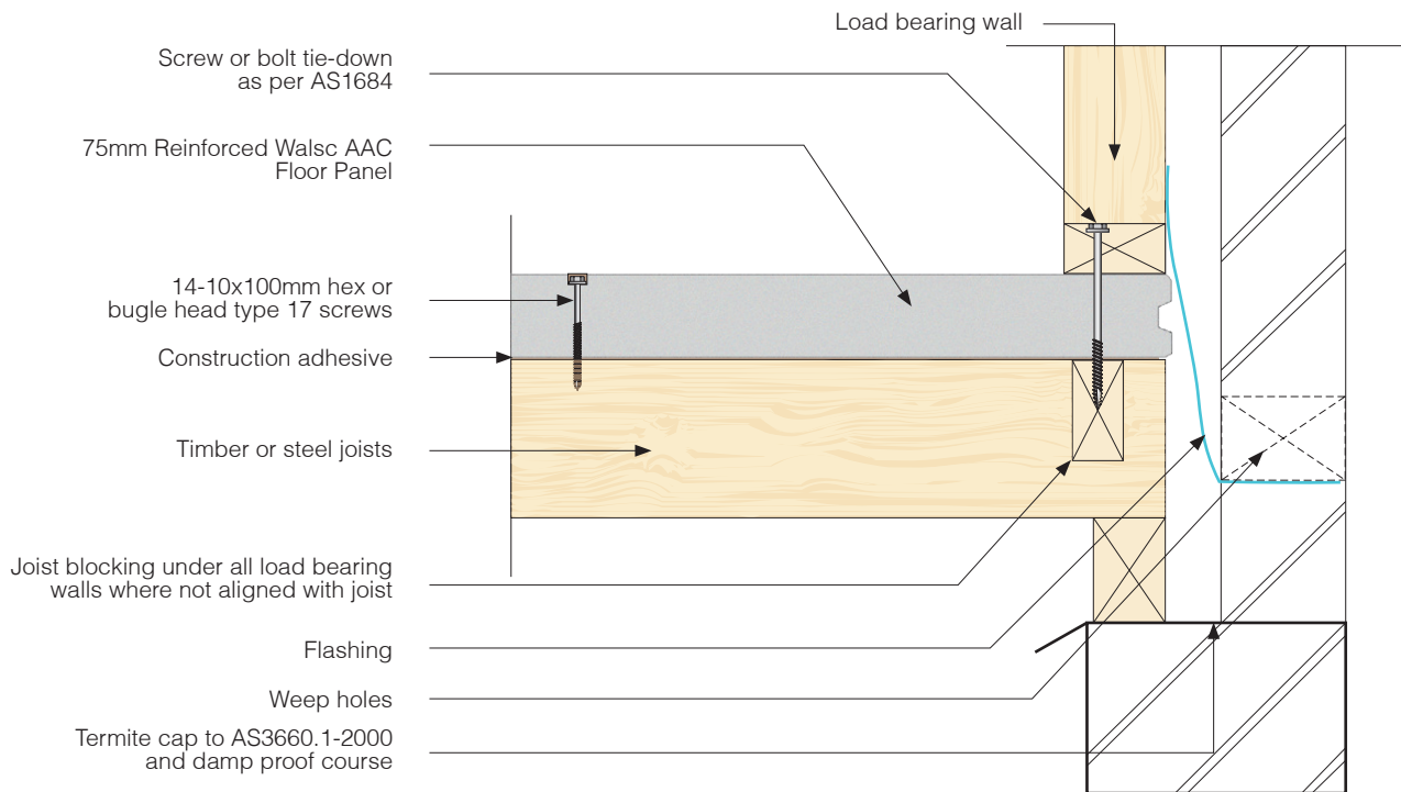
Fig 16. External Brick Veneer Wall Support Detail
