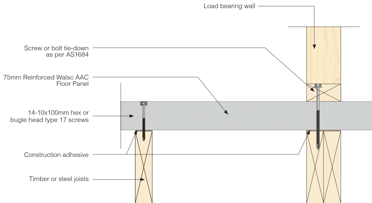
Fig 13. Load Bearing Wall Support Detail on Double Joist
