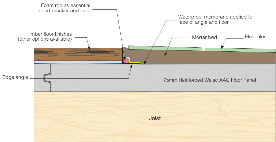
Fig 20. Wet Area Detail
