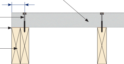
Fig 3. Edge Fixing Detail
