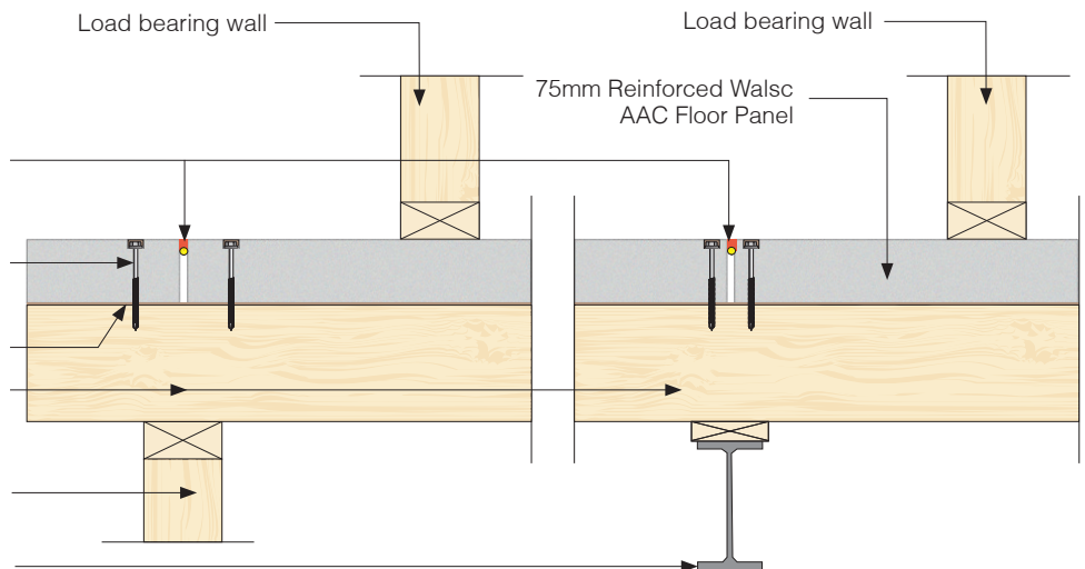
Fig 12. Control Joint Detail Where Joist Span is Supporting Load Bearing Walls
