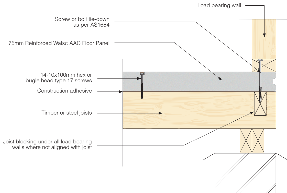
Fig 15. External Wall Support Detail
