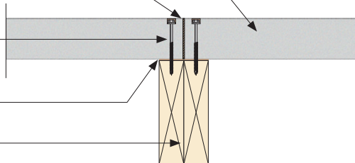
Fig 5. Panel End Joint Fixing Detail on Double Joist
