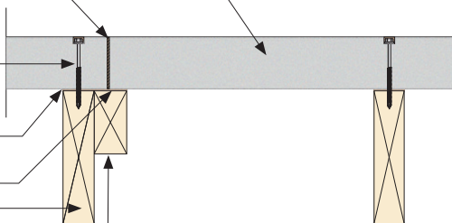
Fig 6. Panel End Joint Fixing Detail on Ledger Plate
