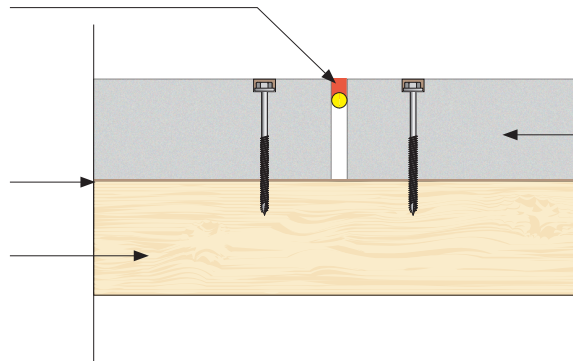
Fig 10. Control Joint Detail
