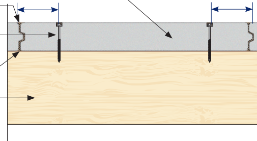
Fig 4. Fixing Detail
