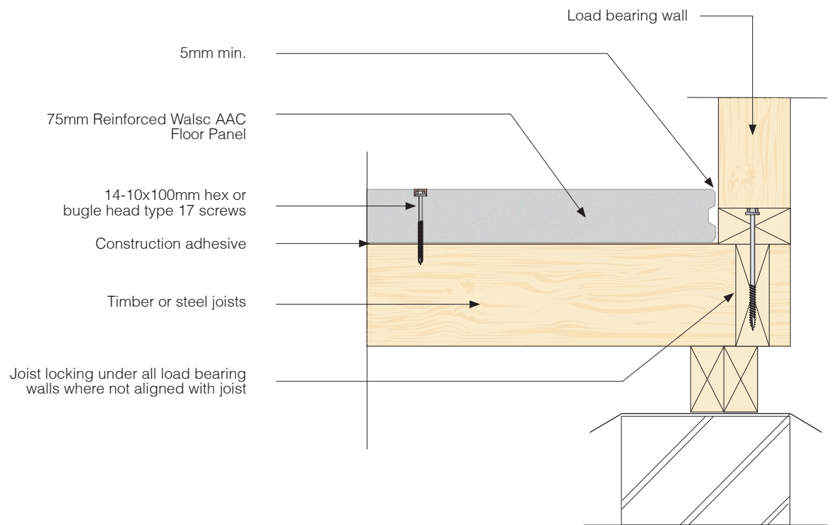
Fig 18. Fitted Floor Panel at External Wall Detail
