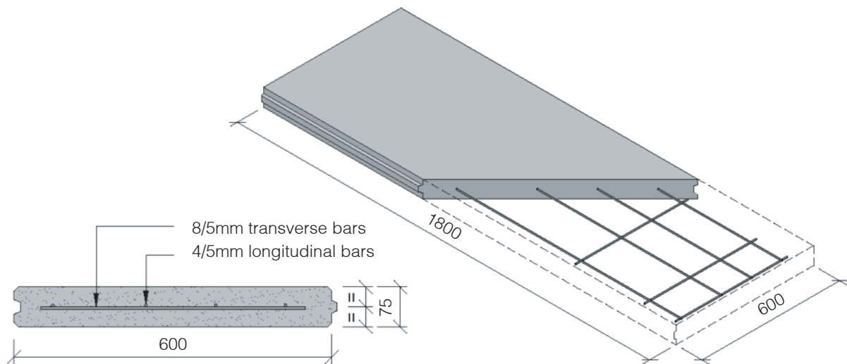
Fig 1. Panel Details
